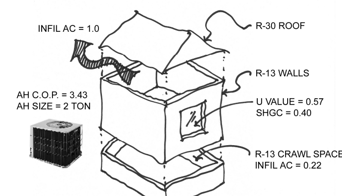
Post 1992 Crawl Space Model
