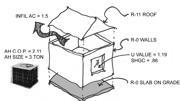
Pre 1978 Slab on Grade Model
