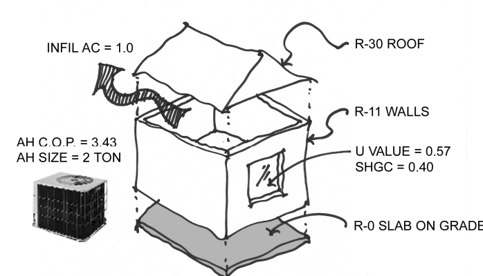
Post 1992 Slab on Grade Model
