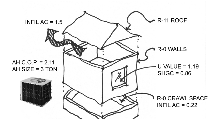
Pre 1978 Crawl Space Model
